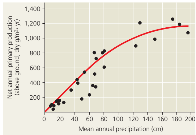
▲ Figure 55.9 A global relationship between net primary production and mean annual precipitation for terrestrial ecosystems.
