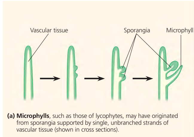
▲ Figure 29.14 Hypotheses for the evolution of leaves.
